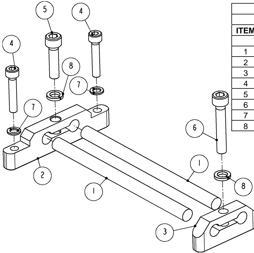
Figure 10 1901430: GUIDE ASSEMBLY
