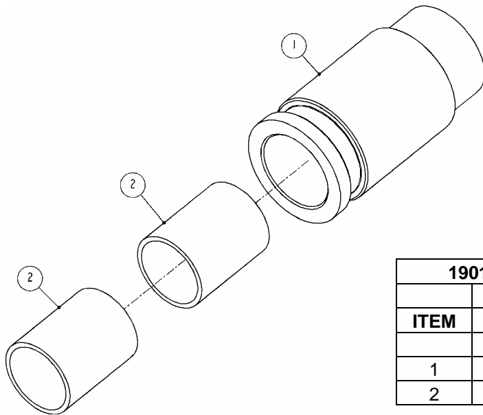
Figure 11 1901500: CARTRIDGE – BEARING ASSEMBLY
