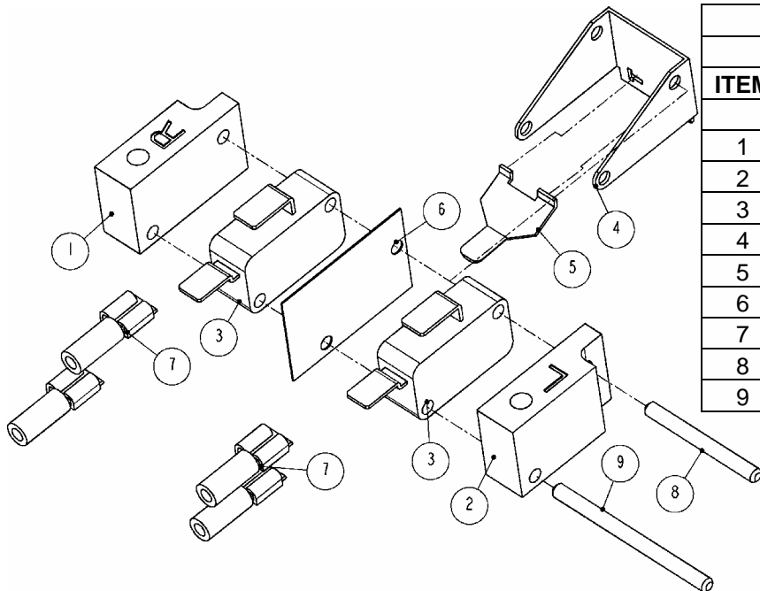
Figure 17 1902600: SWITCH ASSEMBLY
