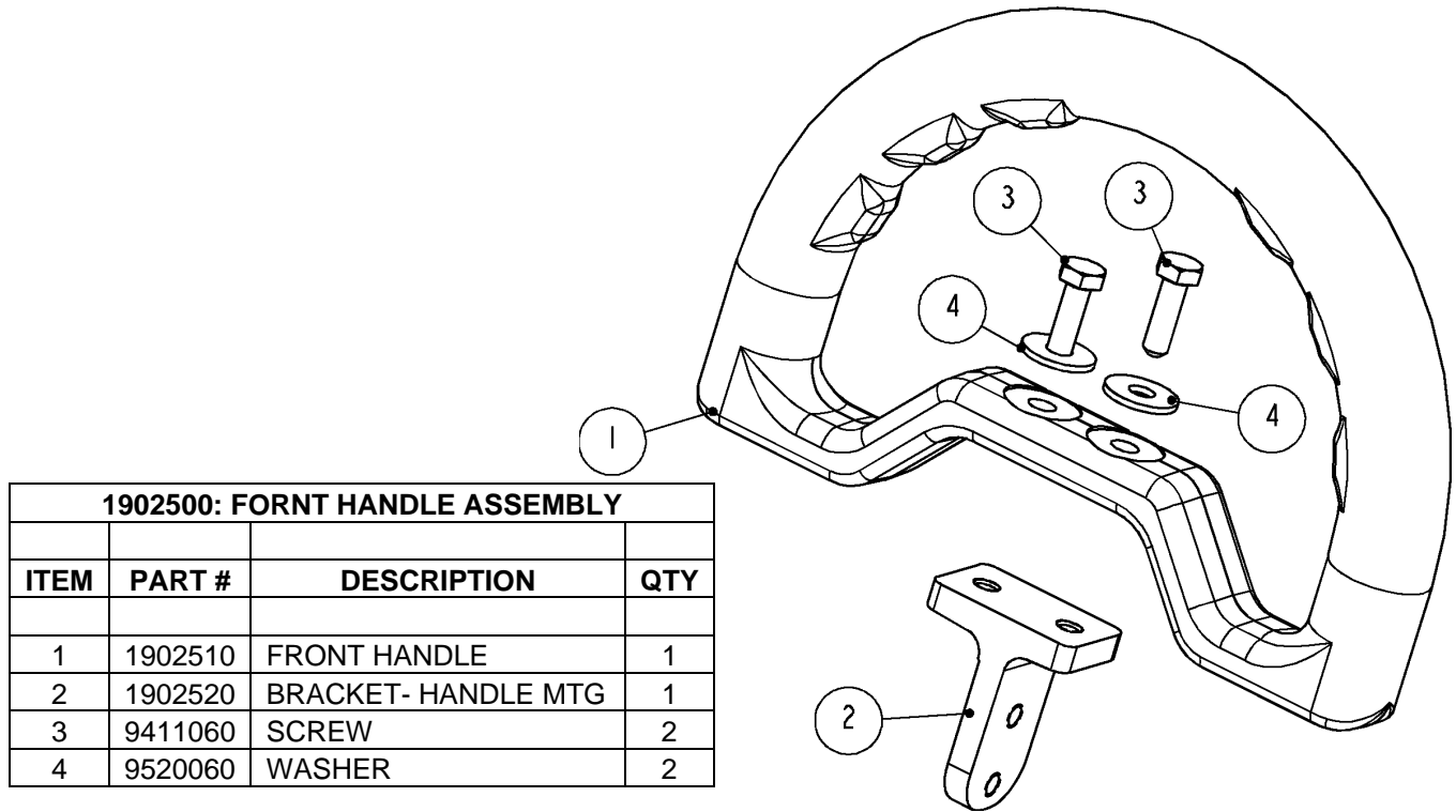
Figure 18 1902500: FRONT HANDLE ASSEMBLY
