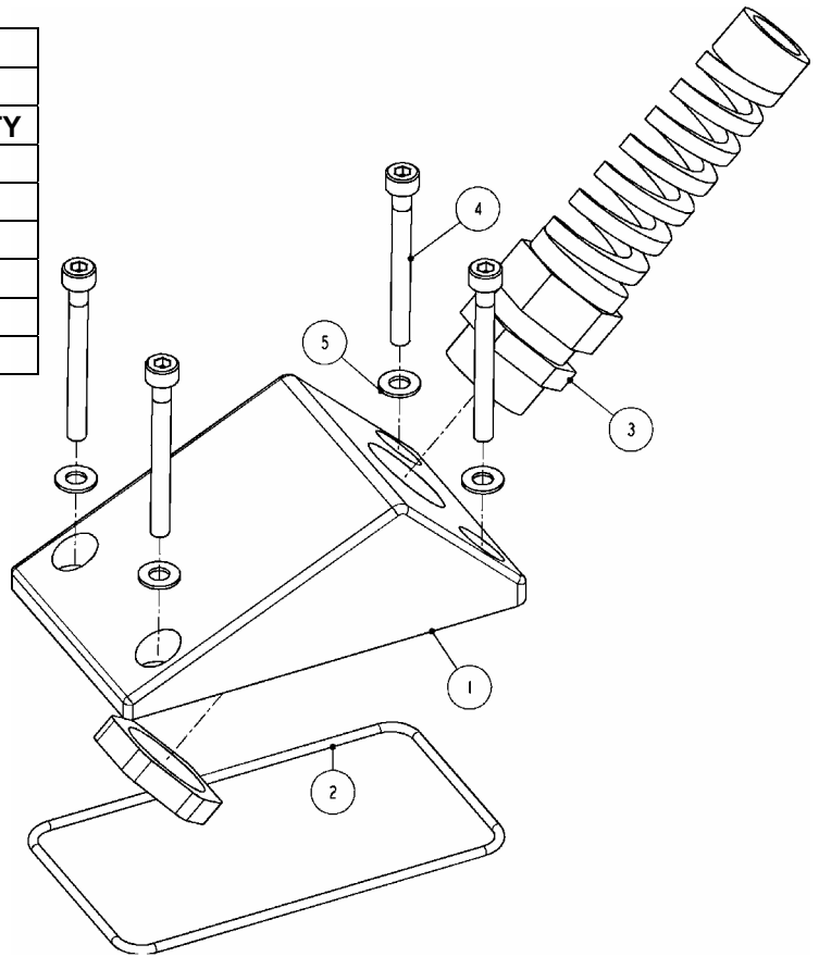
Figure 16 1900900: TOP - REAR HANDLE
