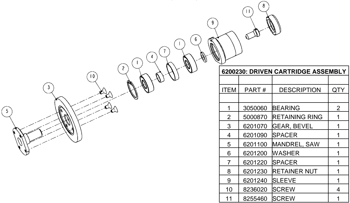
Figure 8 6200230: DRIVEN CARTRIDGE ASSEMBLY
