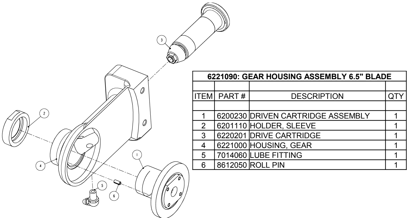
Figure 7 6201250: GEAR HOUSING ASSEMBLY, SC-650
