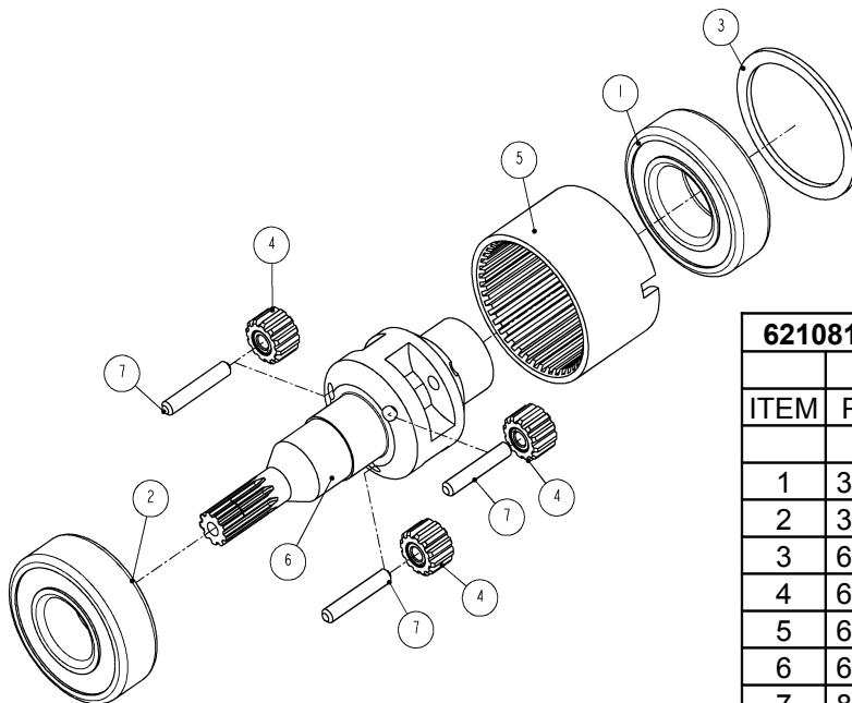
Figure 14 6210800: AIR MOTOR ASSEMBLY, SC-550 & SC-650
