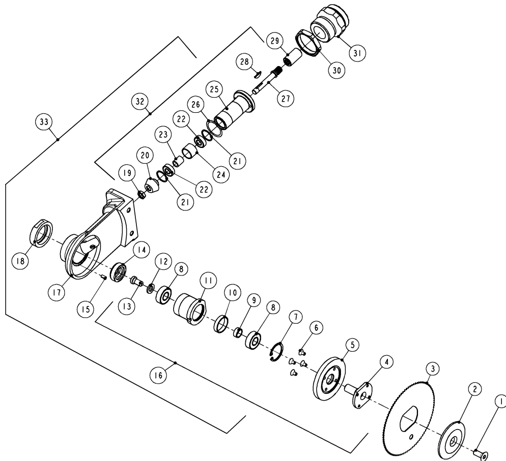
Figure 11 SC-, SPECIAL TOOLS (OPTIONAL)
